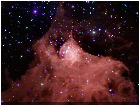
Figure 1.1: Composite image of Cepheus B, a GMC about 2400 Lj away. Red, green & blue data is in infrared, violet in X-Ray spectrum. The image span is about 3 pc.[6]
